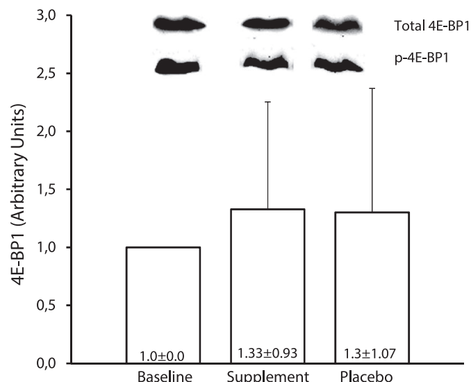
Fig. 4. 4E-BP1 phosphorylated to total protein ratio normalized values to baseline session values ( X \pm SD ). There was no significant change in levels of phosphorylation between any visit ( p > .05 ).
